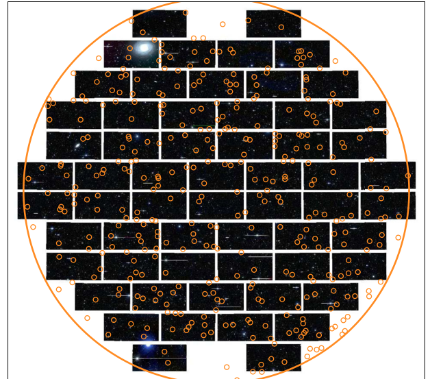
Figure 1. The 2dF spectrograph has 392 optical fibres to be placed at positions across a field of view 2^\circ in diameter (large orange circle). This is well matched to the DECam field of view (image mosaic in the background), making spectroscopic follow-up very efficient. The small orange circles represent the locations of targets selected for one set of AAT observations.
